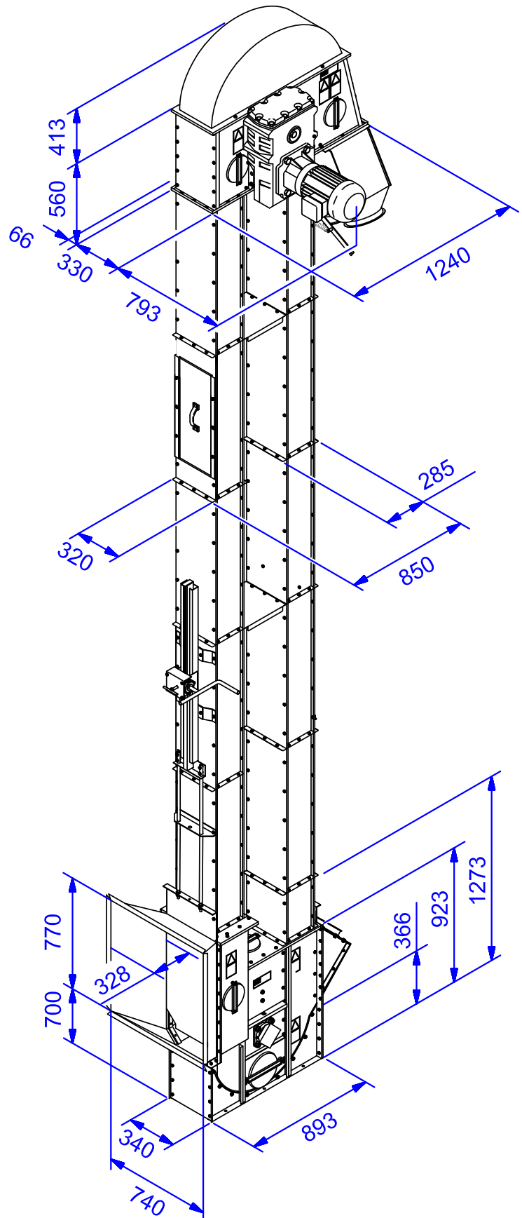
Antti-elevator, E-series, main dimensions
